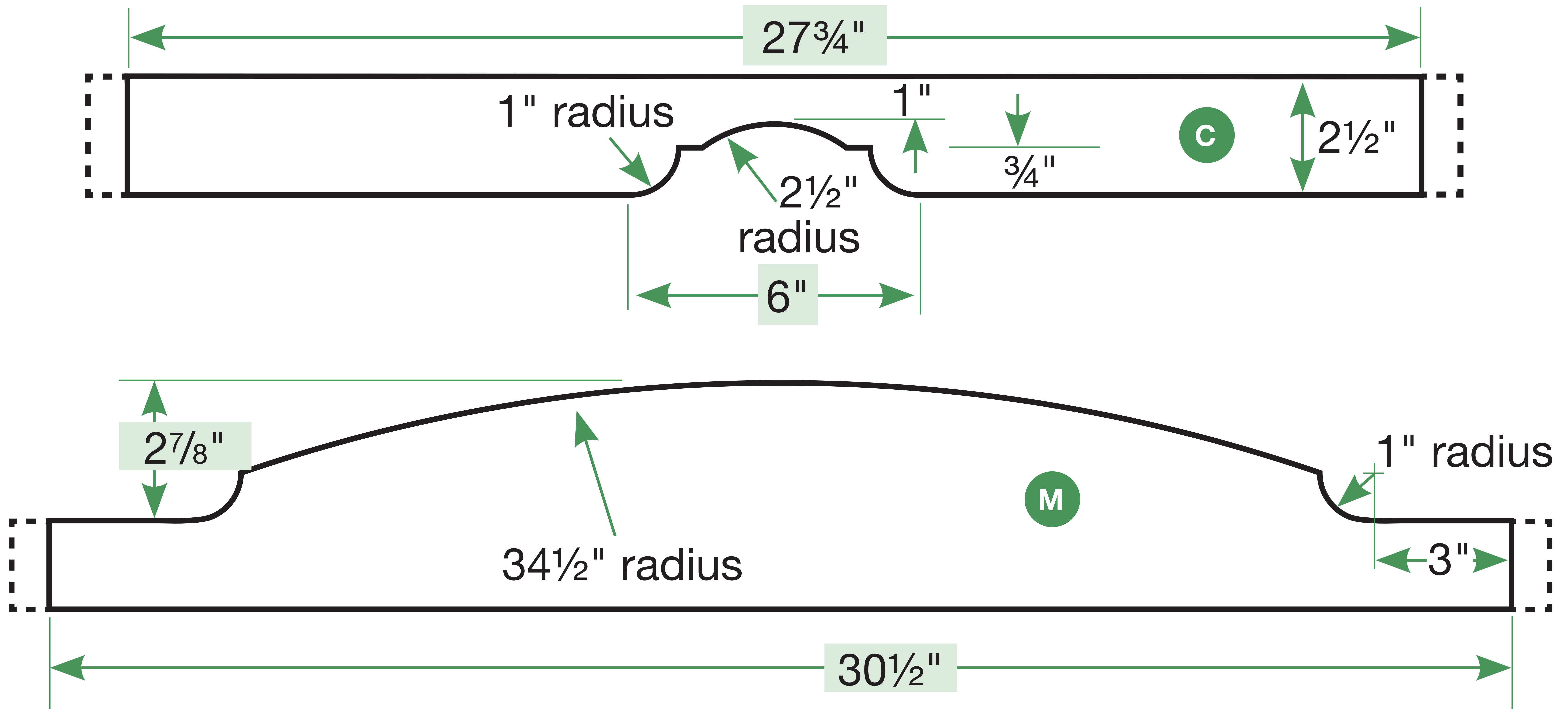
Templates Note: templates extend 1" longer than workpiece where indicated by dotted lines.
